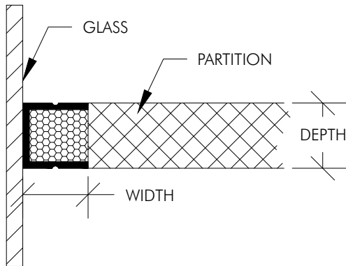
1 THREE SIDE COATED EXAMPLE N.T.S.
